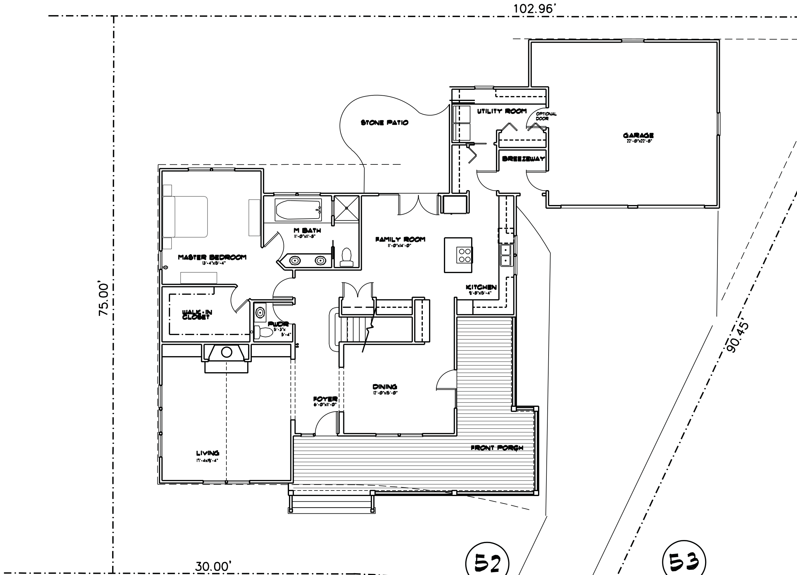
MAIN LEVEL FLOOR PLAN
