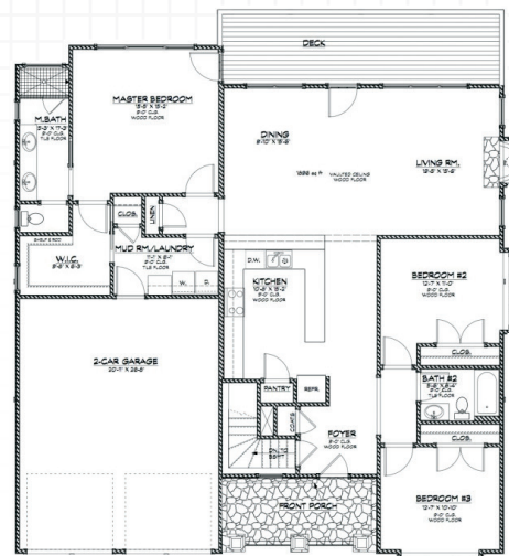
3 Bedroom floorplan option
