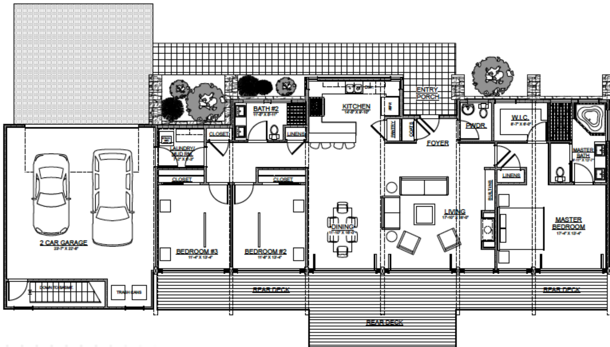
THE ZEPHYR - FIRST FLOOR PLAN Scale: 1/4" = 1'-0" ©2015 RETRO+FIT DESIGN L.L.C. TOTAL HEATED/FINISHED SQUARE FOOTAGE = 1957 S.F.
